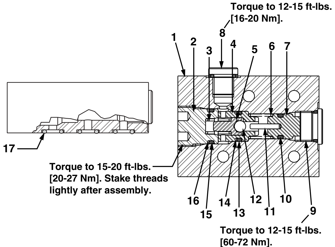
Repair Parts List for Figure 2 — MVM-72
