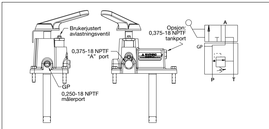
Figur 1, Pumpemontert VM32
