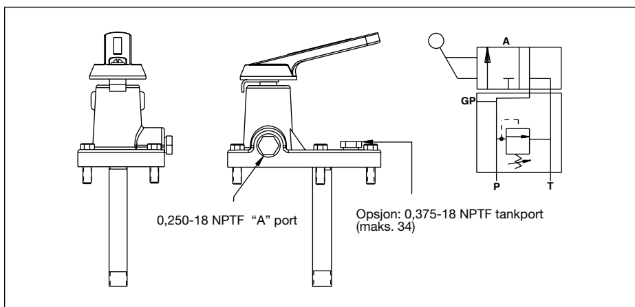
Figur 3, Pumpemontert VM2
