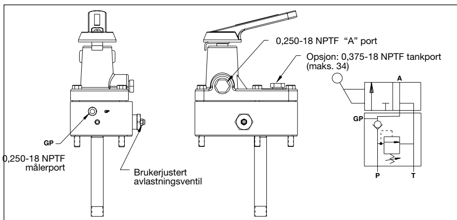
Figur 2, Pumpemontert VM22
