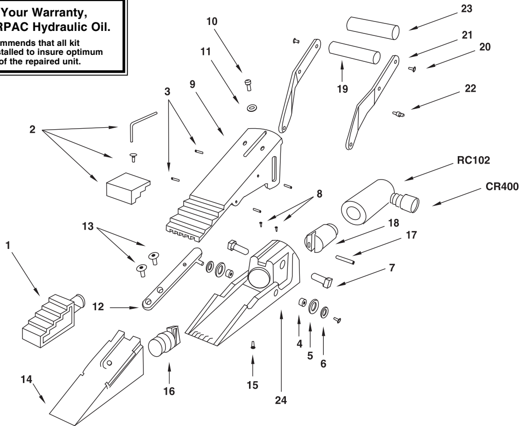
Figure 1, Lifting Wedge Assembly
