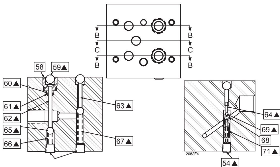
Fig. 4 Valve Body
