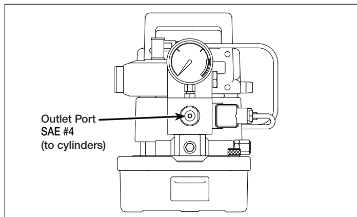
Figure 3, Control Valve Outlet Port
