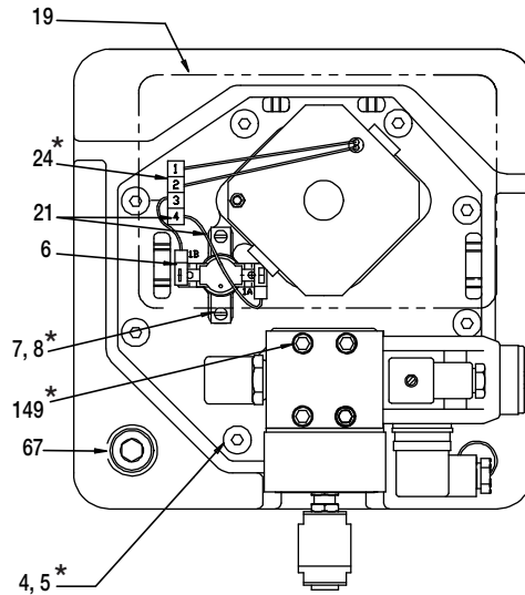
Figure 6, Pump Top View (shroud removed)
