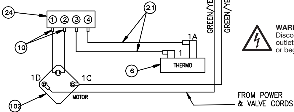
Figure 14, Wiring Diagram, Motor and Thermostat
