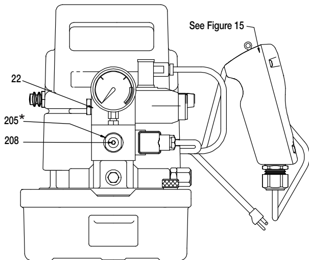
Figure 5, Pump Front View (shroud installed)
