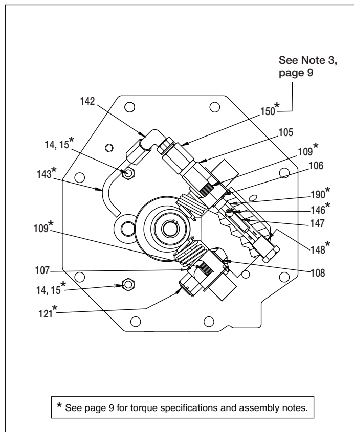
Figure 4, Pump Bottom View
