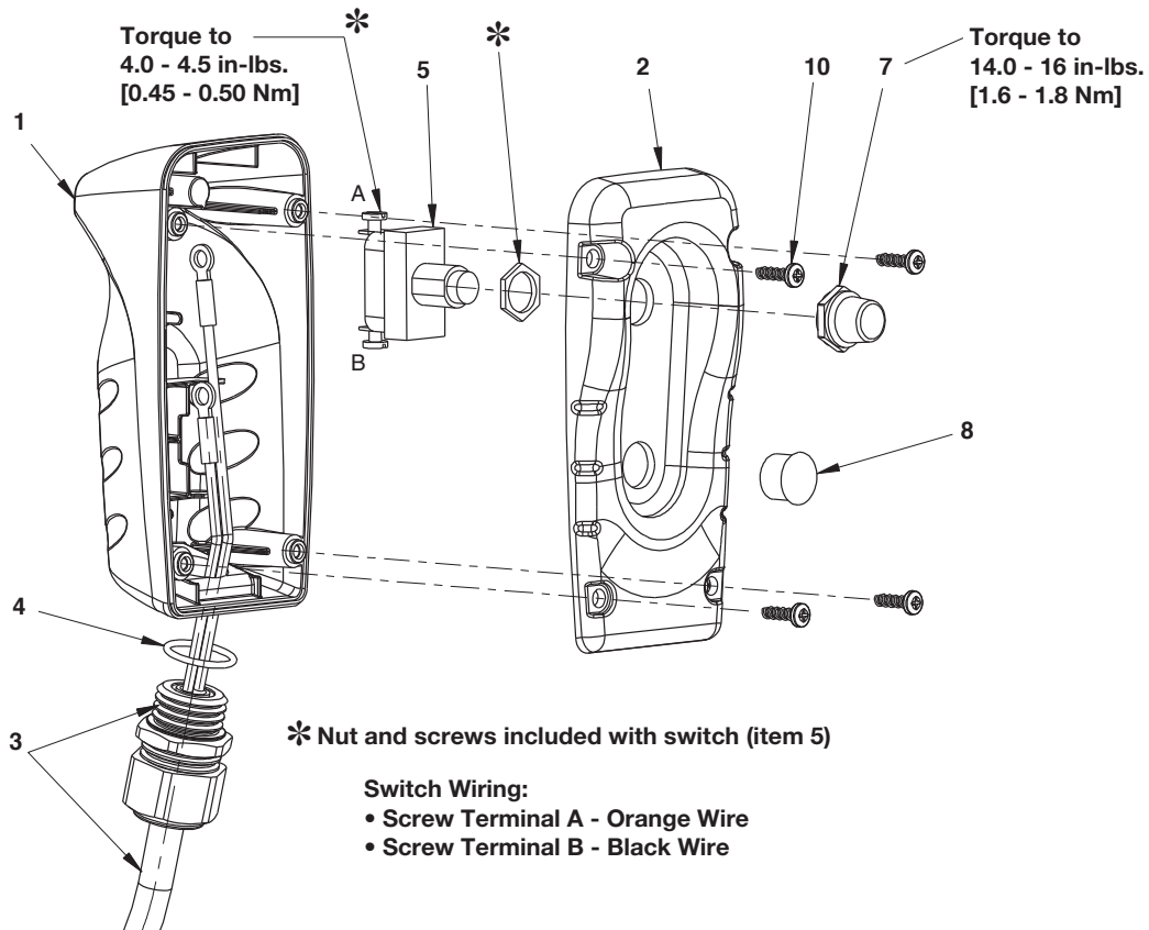
Figure 15, Remote Pendant Assembly
