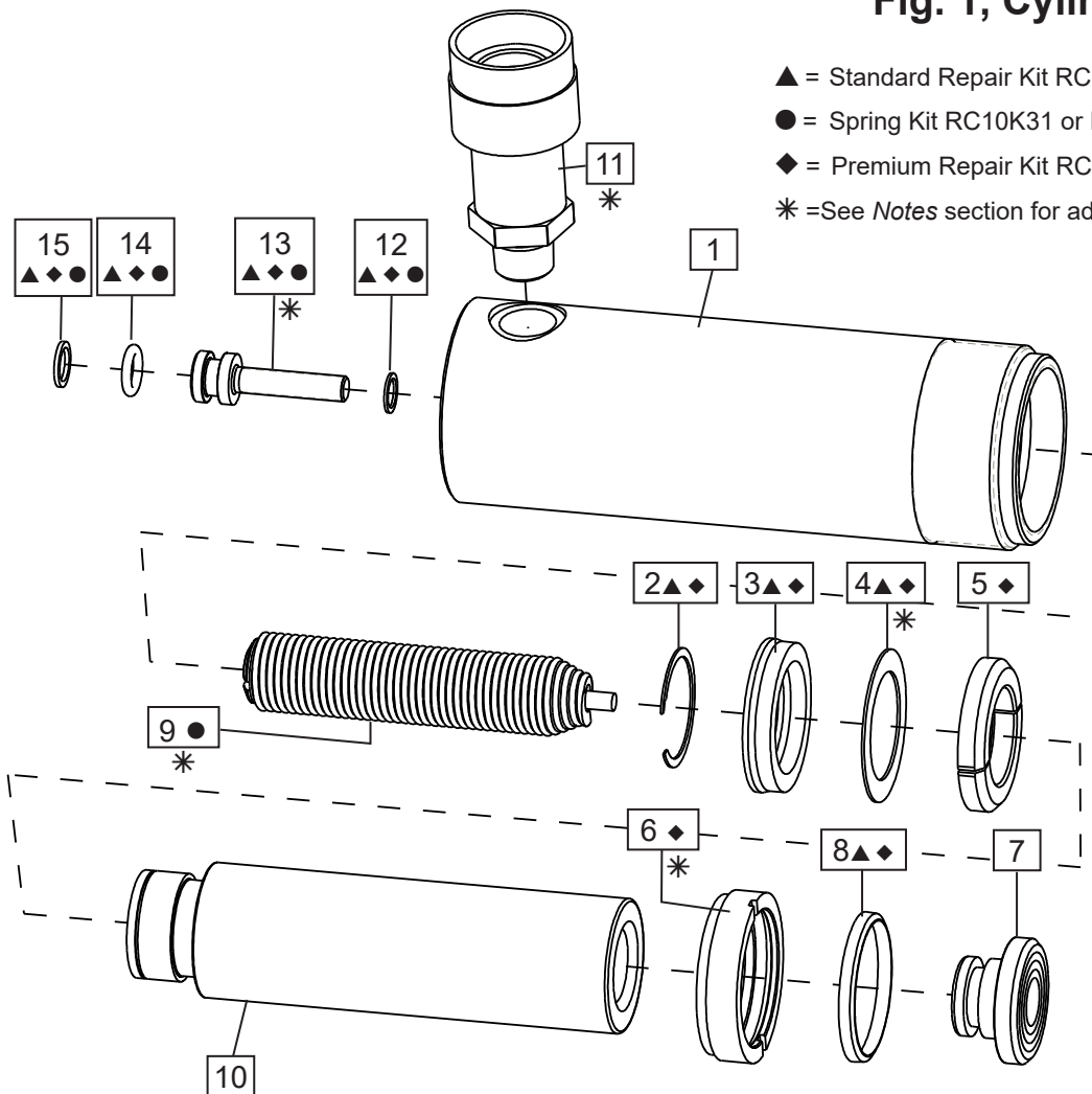
Fig. 1, Cylinder Assembly
