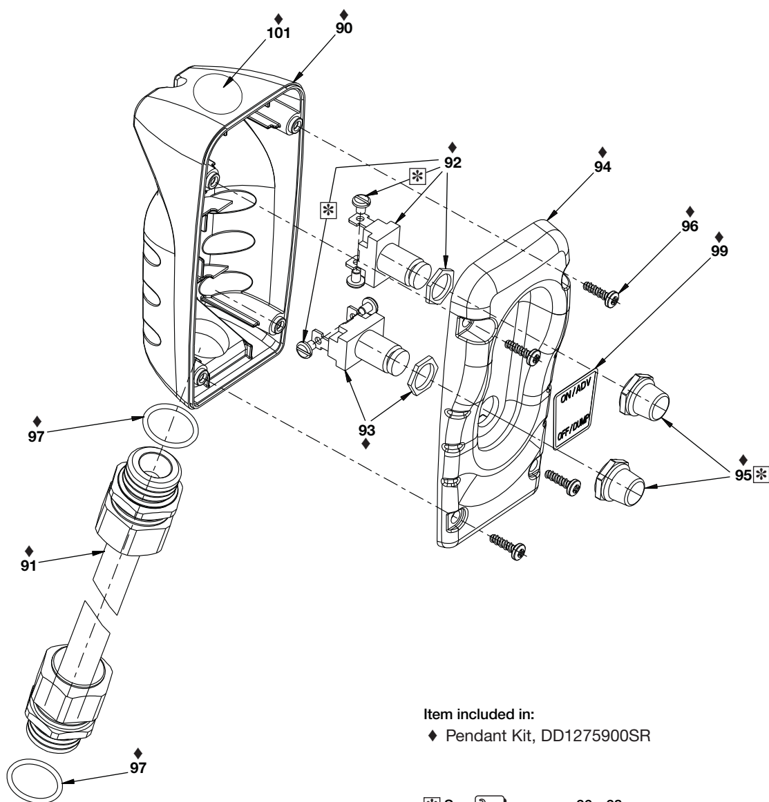
Figure 7, Pendant and Cable Assembly, 2-Button
