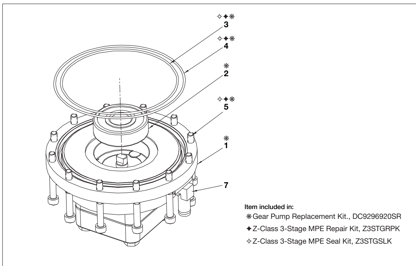
Figure 18, Gear Pump and O-Rings
