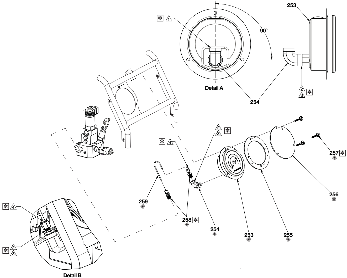
Figure 3, Pressure Gauge Assembly
