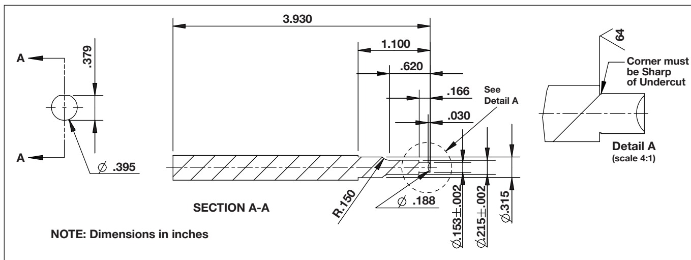
Figure 17, Seat Tool Drawing
