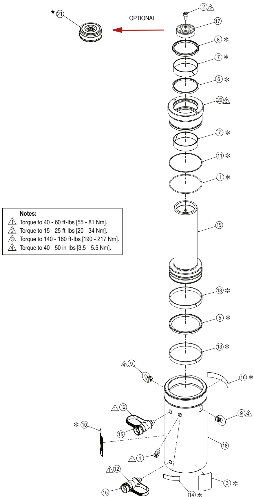
Figure 4, Exploded View - Model HCR-100 Tall
