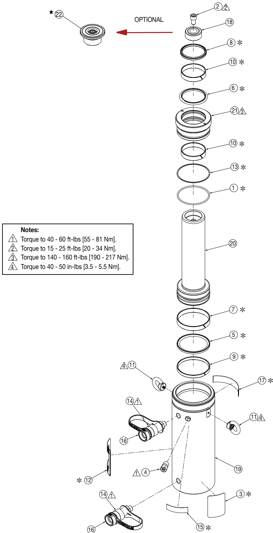
Figure 2, Exploded View - Model HCR-50 Tail
