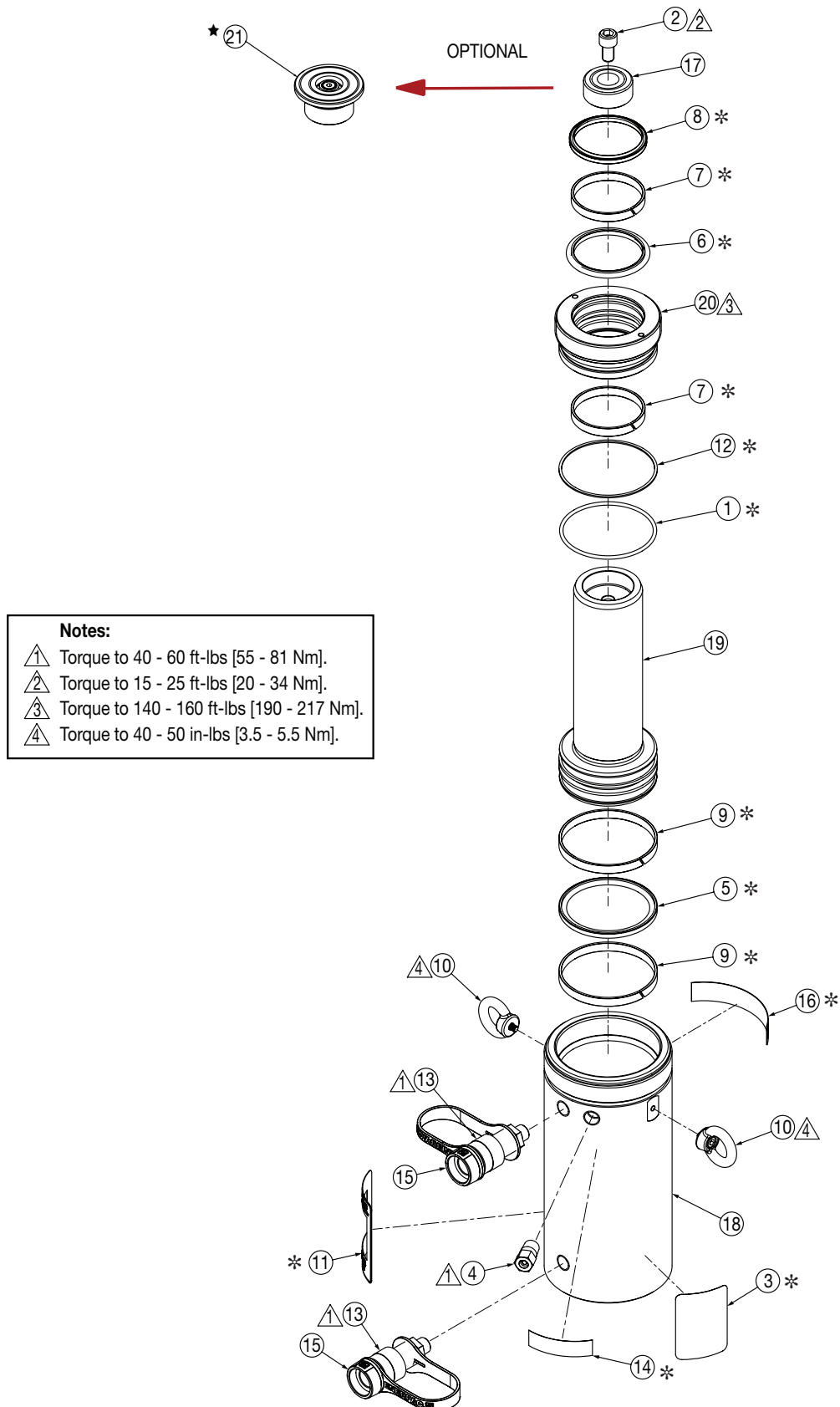
Figure 1, Exploded View - Model HCR-50 Short
