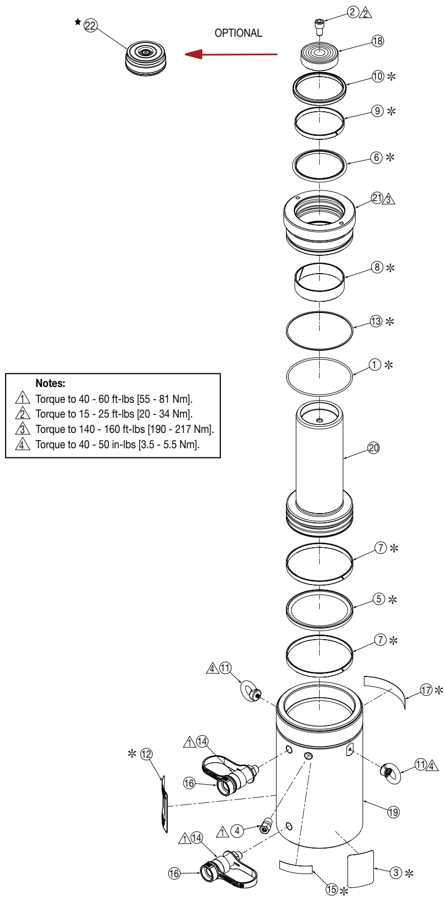
Figure 3, Exploded View - Model HCR-100 Short
