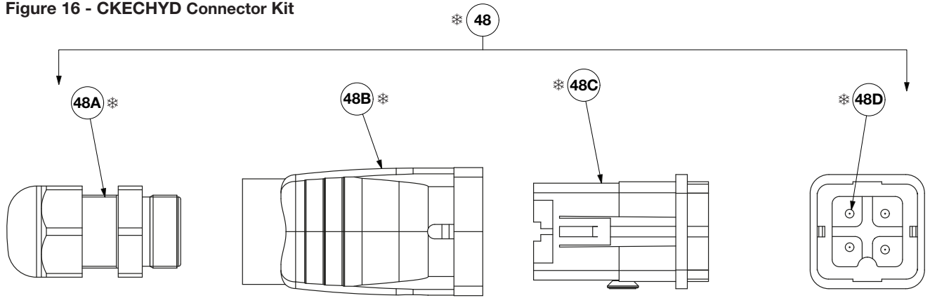
Figure 16 - CKECHYD Connector Kit
