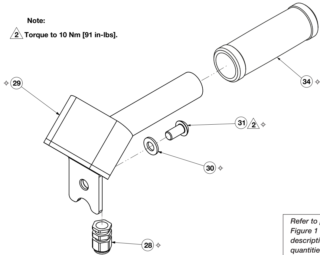
Figure 13 - EBH5205K Handle Kit
