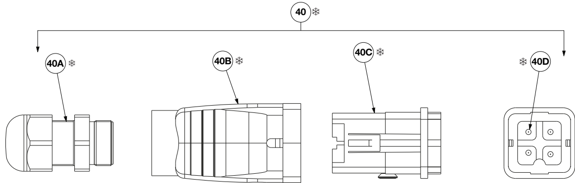
Figure 16 - CKECHYD Connector Kit
