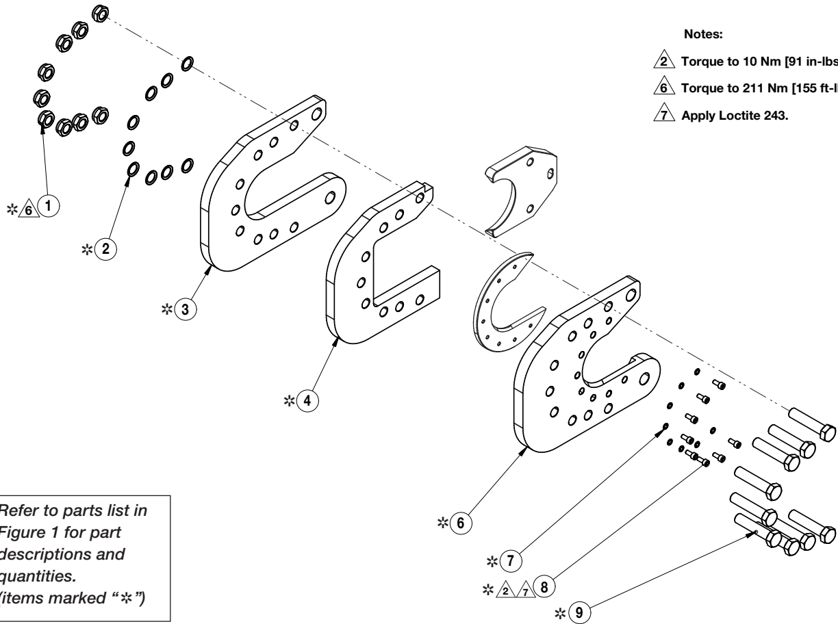
Figure 4 - EWCH9003K Guide Kit
