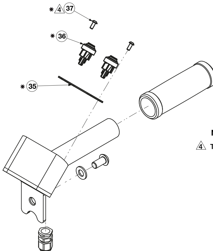
Figure 12 - EBH5204K Switches Kit
