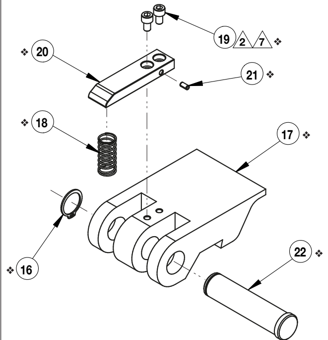
Figure 6 - EWCH9005K Latch Kit
