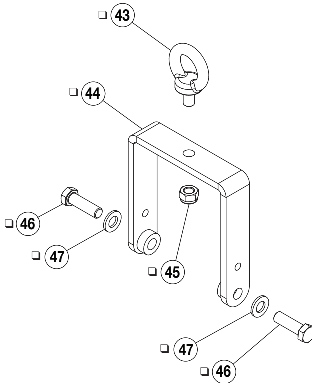
Figure 11 - EWCH9010K Lift Kit
