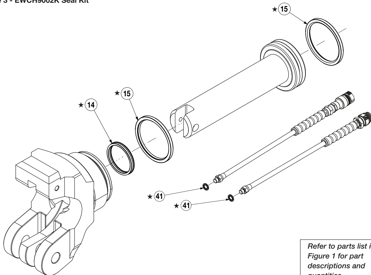
Figure 3 - EWCH9002K Seal Kit
