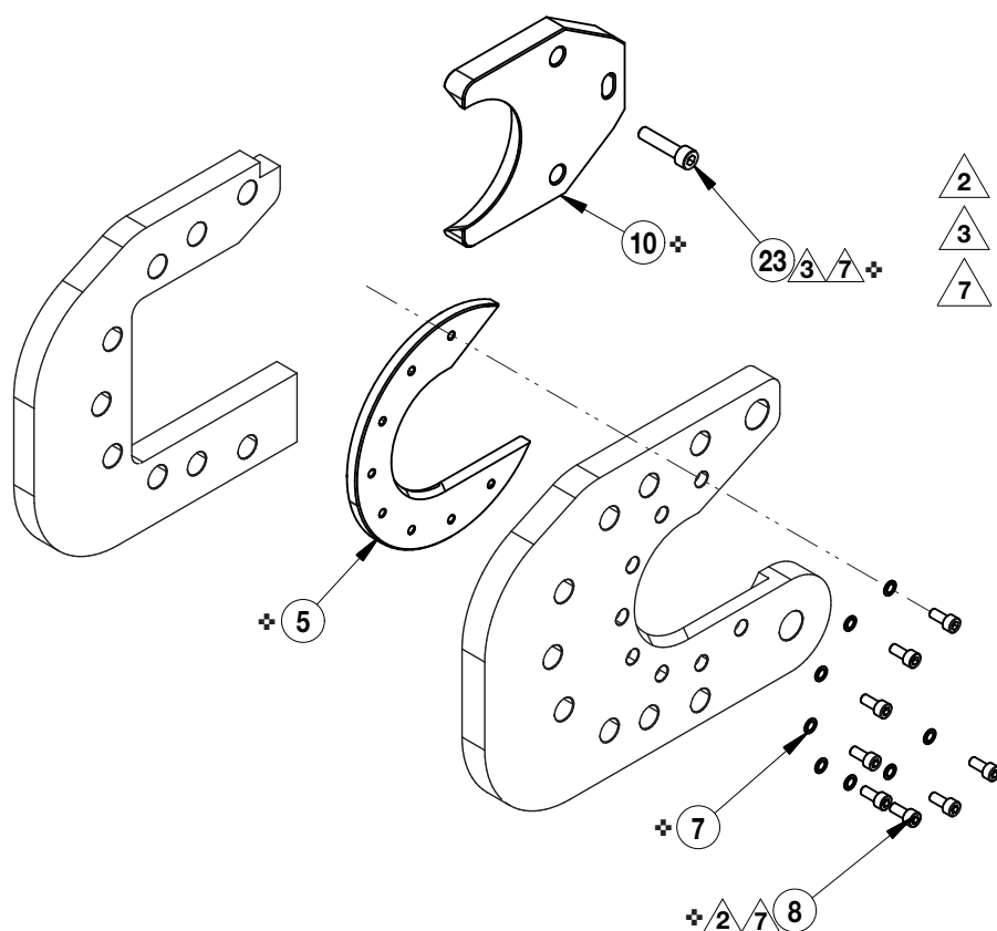
Figure 2 - EWCH9001K Blade Kit
