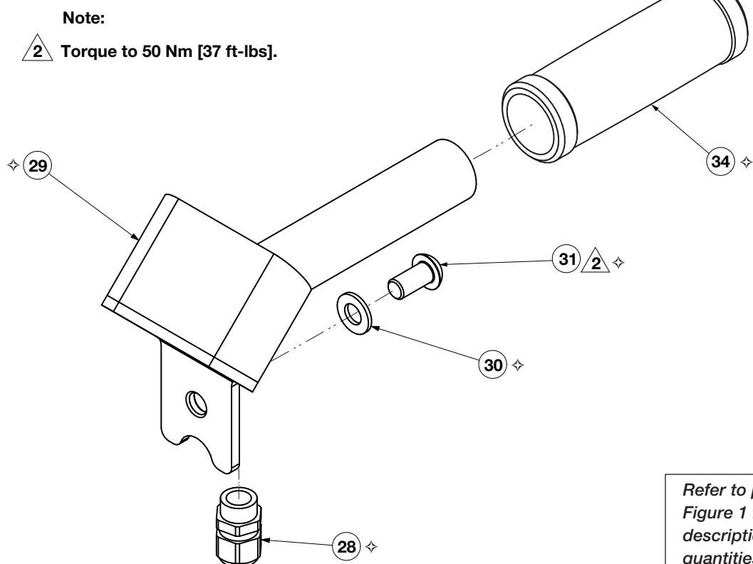
Figure 12 - EBH5205K Handle Kit
