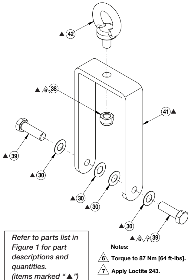
Figure 5 - EWCH14004K Lift Kit
