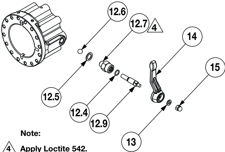
Figure 10 - EFBE501707K Release Valve Kit
