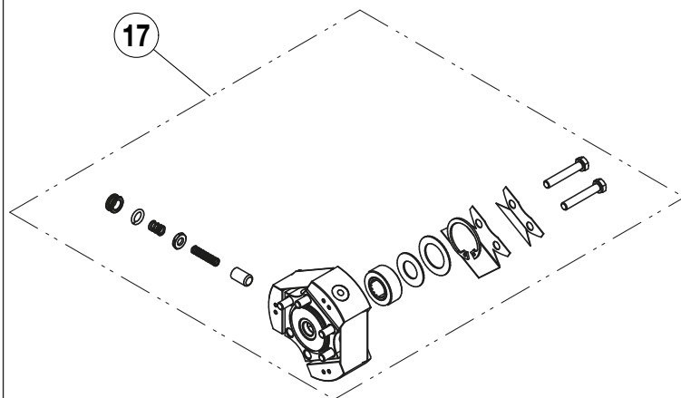
Figure 8 - EBE2210K Pump Kit
