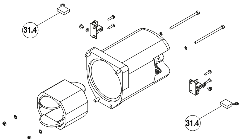
Figure 15 - EBE2222K and EBE2215K Brush Kit
