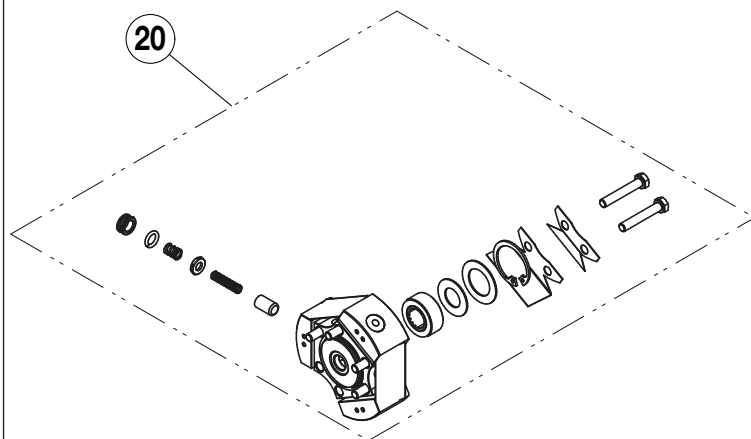
Figure 10 - EBE2210K Pump Kit
