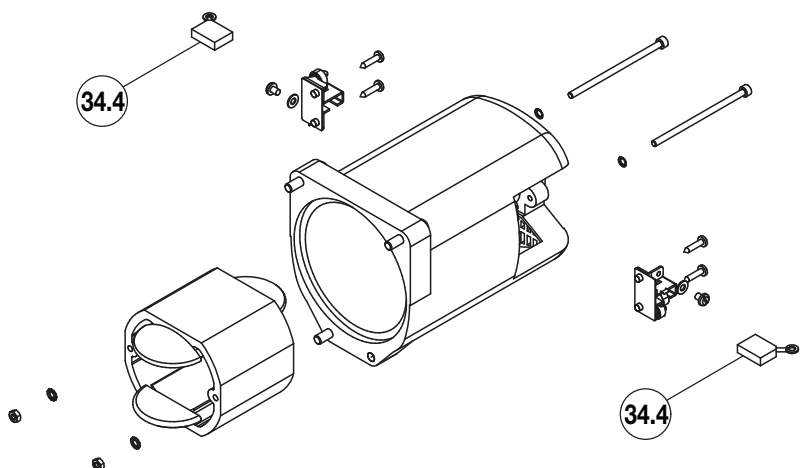
Figure 17 - EBE2222K and EBE2215K Brush Kit
