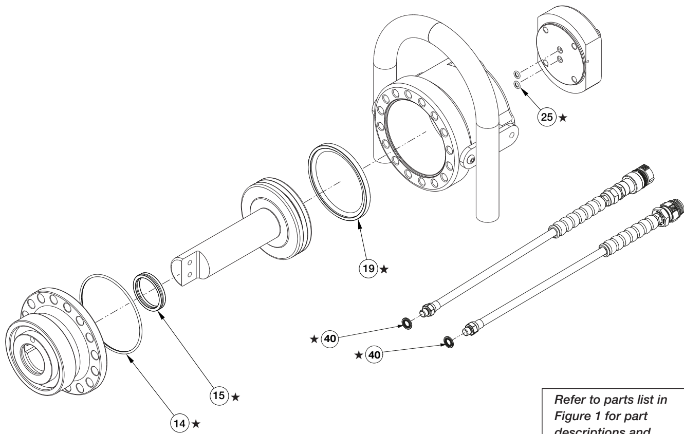
Figure 3 - EBH3002K Seal Kit
