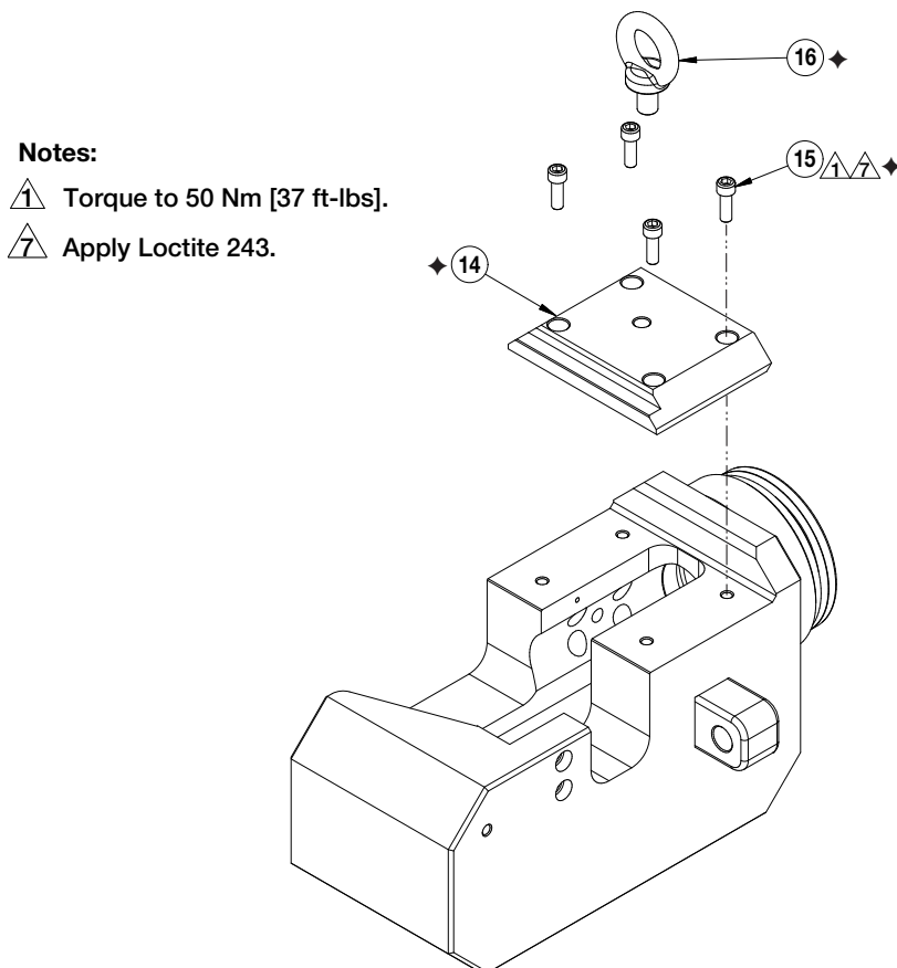
Figure 10 - EBH5210K Top Cover Kit
