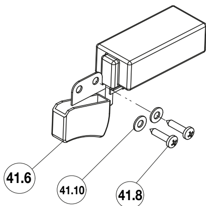
Figure 13 - EBE2223K & EBE2203K Switch Kit
