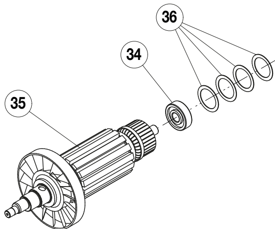
Figure 15 - EBE2211K & EBE2220K Rotor Kit
