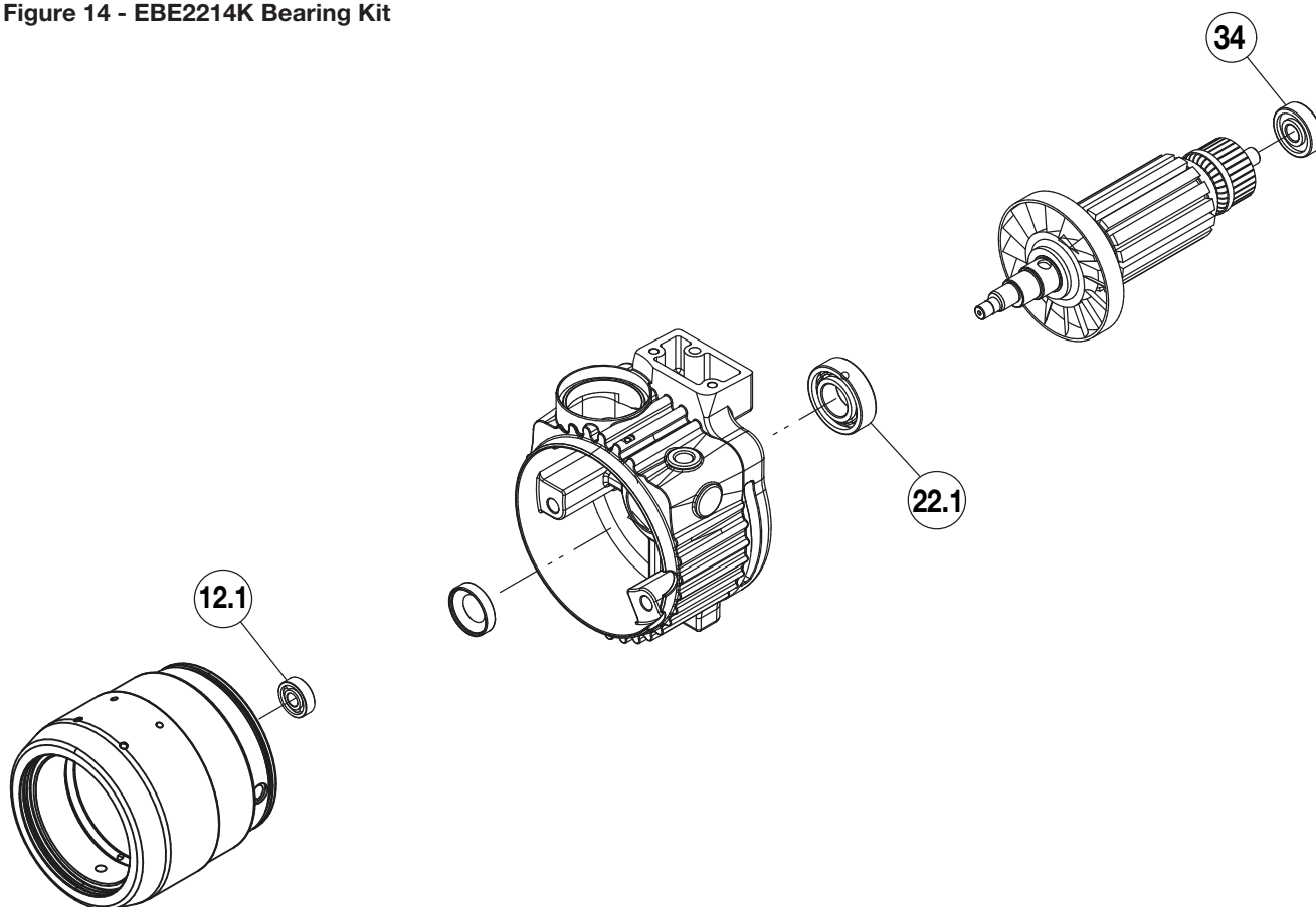
Figure 14 - EBE2214K Bearing Kit
