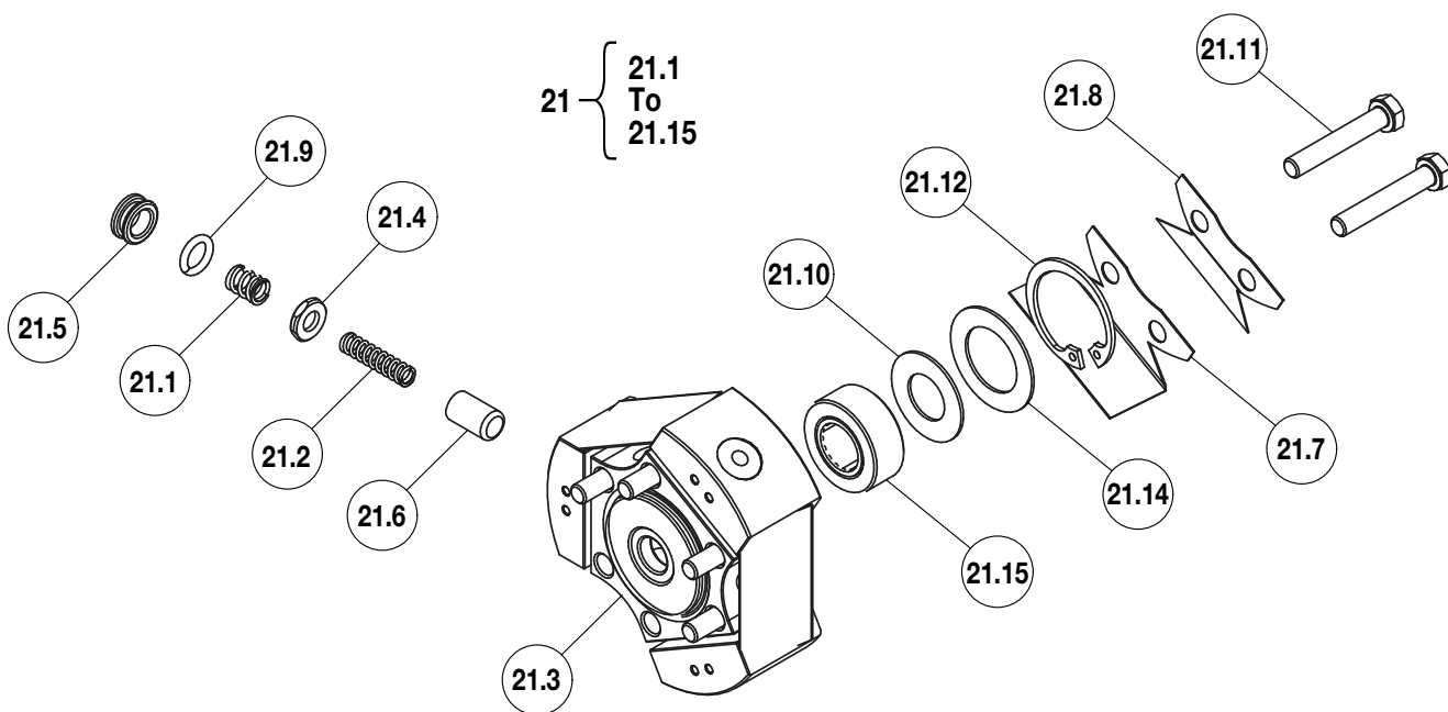
Figure 10 - EBE2210K Pump Kit
