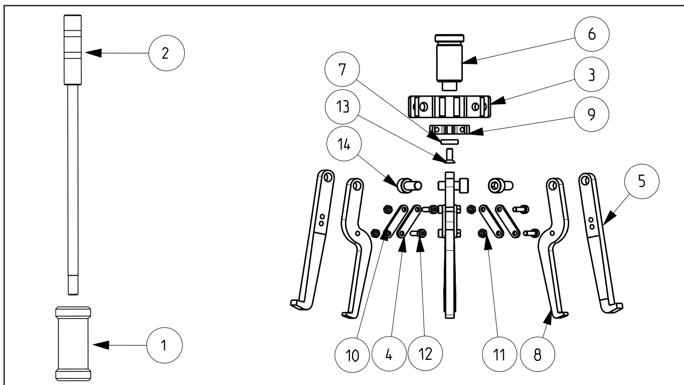
Figure 1, Mechanical Internal Puller Assembly, IPM3
